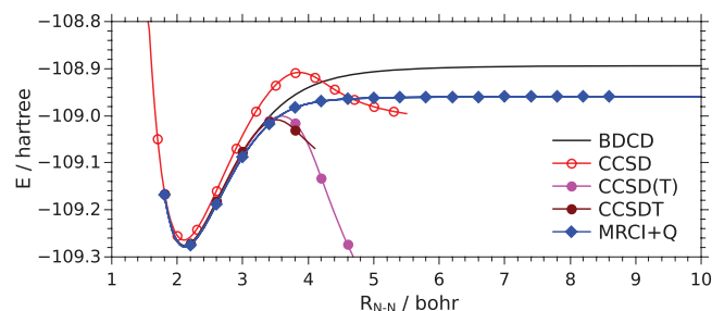
FIG. 2. Potential energy curves for N_2 dissociation.
