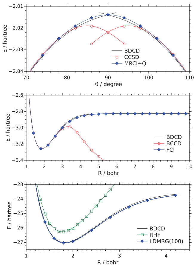
FIG. 3. Potential energy curves for hydrogen systems. (Top) H_4 system with geometry from Ref. 25 (see text). (Middle) Uniform dissociation of hexagonal H_6 , in which R is the distance of each hydrogen atom from the centre. (Bottom) Uniform dissociation of H_{50} chain, with comparison to DMRG calculations from Ref. 26.
