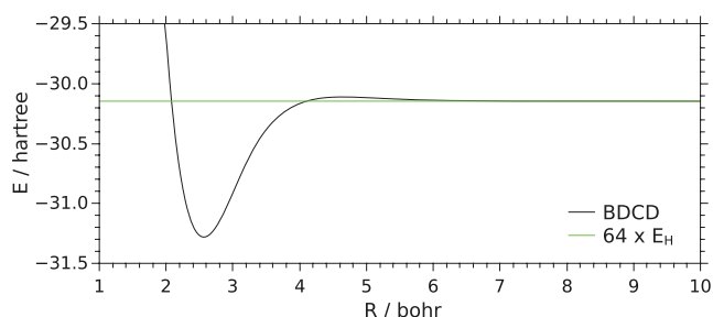
FIG. 4. Uniform dissociation of 4 \times 4 \times 4 cube of hydrogen atoms, a model for incipient strong correlation in the metal-insulator transition.
