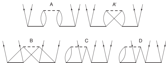
FIG. 1. Nonantisymmetrized Goldstone diagrams contributing to the CCD amplitude equation that are quadratic in the amplitudes. The solid interaction lines denote a T_2 amplitude; the dashed lines a Coulombic interaction from the Hamiltonian; and the thin lines particles (downward arrows) or holes (upward arrows) in the spin-orbital representation.
