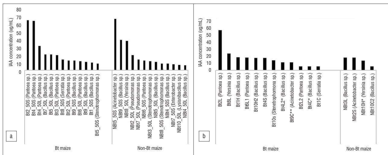
Figure 7: Estimated indole acetic acid (IAA) production of Bt and non-Bt maize endophytes in (a) 50-day-old maize isolates and (b) 90-day-old maize isolates.
