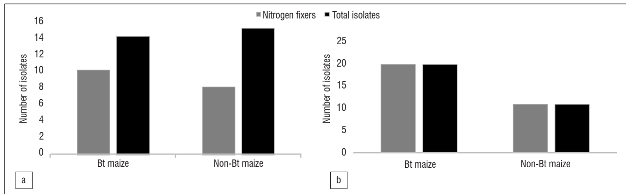
Figure 6: Total number of isolates which were shown to be potential nitrogen fixers in (a) 50-day-old maize isolates and (b) 90-day-old maize isolates.
