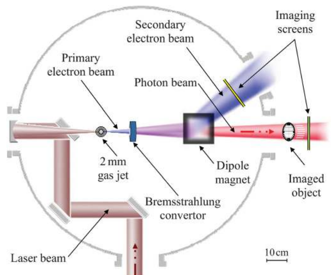
FIG. 1. (Color online) Lay-out of the experimental setup.
