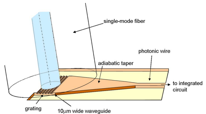
Fig. 1. Coupling principle between fiber and photonic wires by means of a grating.
