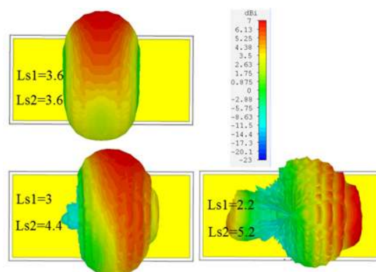
Fig. 18. Simulated 3D radiation patterns of the planar array in different states at 27 GHz.
