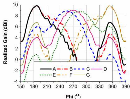
Fig. 6. Simulated radiation patterns of the proposed beam steerable array in different states in the plane of \theta = 72^\circ at 28.5 GHz.
