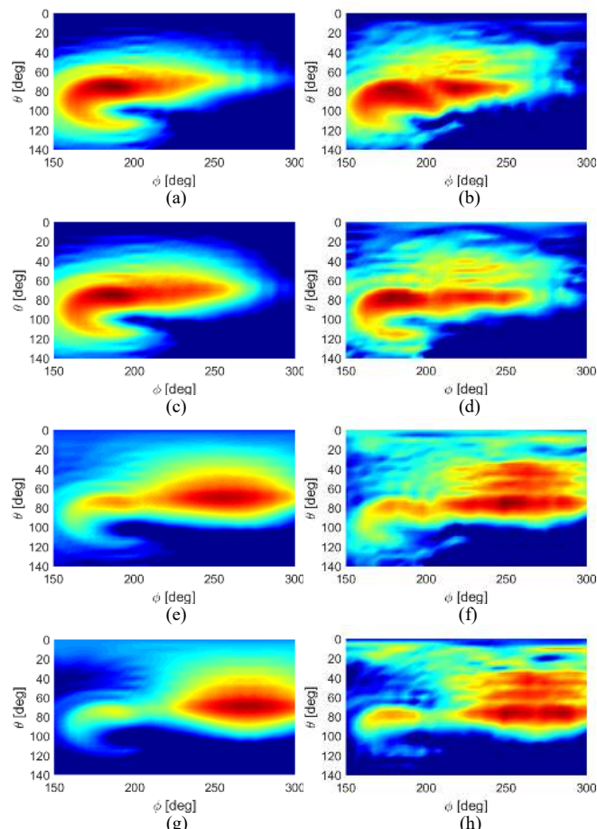
Fig. 21. Simulated 3-D radiation gain patterns of: (a) State A, (c) State B, (e) State C, and (g) State D; measured 3-D radiation gain patterns of: (b) State A(d) State B, (f) State C, and (h) State D. (The color bar is same to that in Fig. 8)
