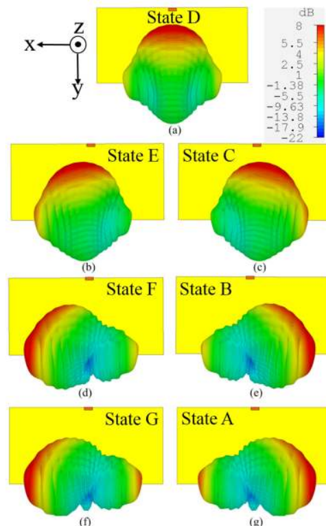
Fig. 5. Simulated 3D radiation patterns of the proposed beam steerable array in different states at 28.5 GHz.
