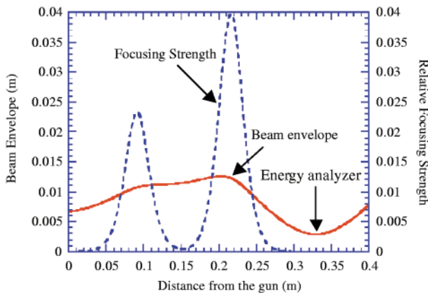
FIG. 7. (Color) Typical beam envelope in the transport line.
