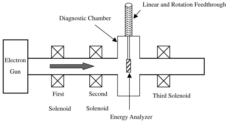
FIG. 6. Experimental setup for the energy analyzer test.
