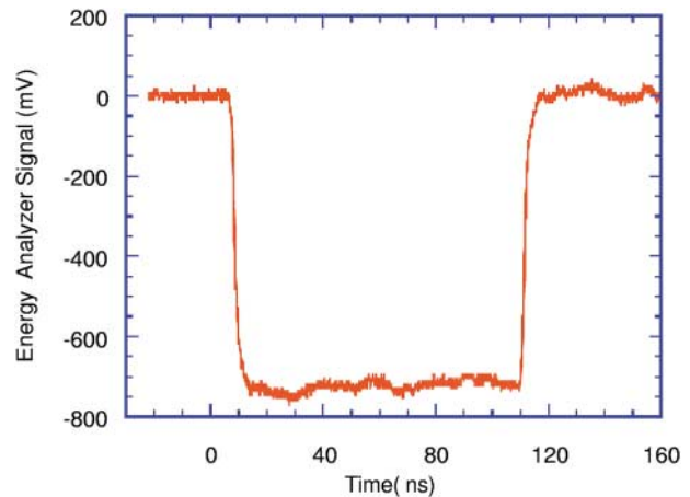
FIG. 8. (Color) Typical energy analyzer output signal.
