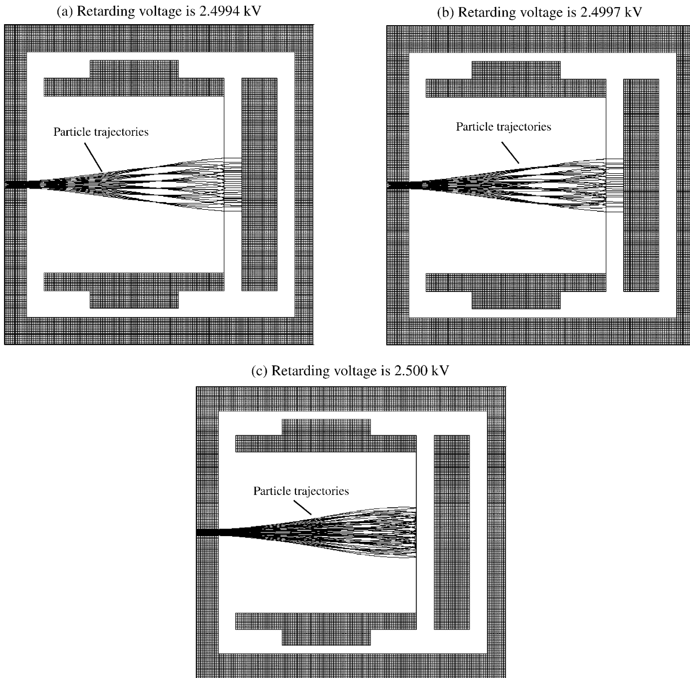
FIG. 3. Particle trajectories at different retarding voltages.
