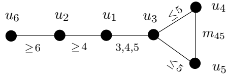
Figure 4.11: A diagram \Sigma' , see Lemma 4.15
