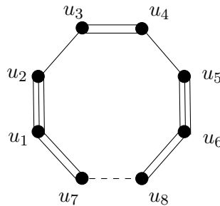
Figure 4.9: Coxeter diagram of a unique Coxeter polytope with Gale diagram G_{12221}
