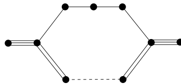
Figure 4.3: Coxeter diagram of a unique Coxeter polytope with Gale diagram G_{12321}
