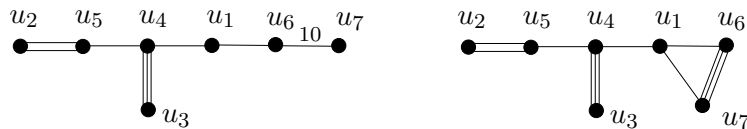
Figure 4.10: All possibilities for diagram \Sigma' , see Lemma 4.9
