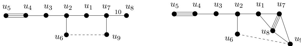
Figure 4.6: Coxeter diagrams of Coxeter polytopes with Gale diagram G_{21411}
