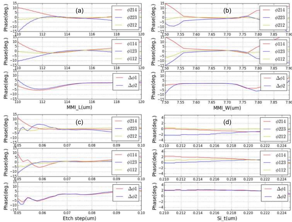
Fig. 3. Tolerance analysis on the phase relations of the ultra-compact 90^\circ hybrid used in this work. (a) Influence of the length of the MMI coupler; (b) influence of the MMI width; (c) influence of the MMI etch depth; (d) influence of the silicon waveguide thickness (1550 nm wavelength, TE polarization).
