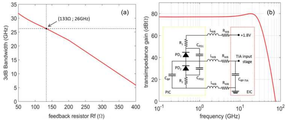
Fig. 7. (a) Simulation of the TIA bandwidth as a function of the trans-impedance with indication of the used transimpedance setting ( 133 \Omega ) and resulting 3 dB-bandwidth (26 GHz). (b) Simulated trans-impedance gain of the TIA as a function of frequency for a trans-impedance of 133 \Omega , as is used in the experiment. The equivalent circuit of the balanced photodiodes taking into account the parasitic capacitance of the pads and the inductance of the bond wire is shown in the inset.
