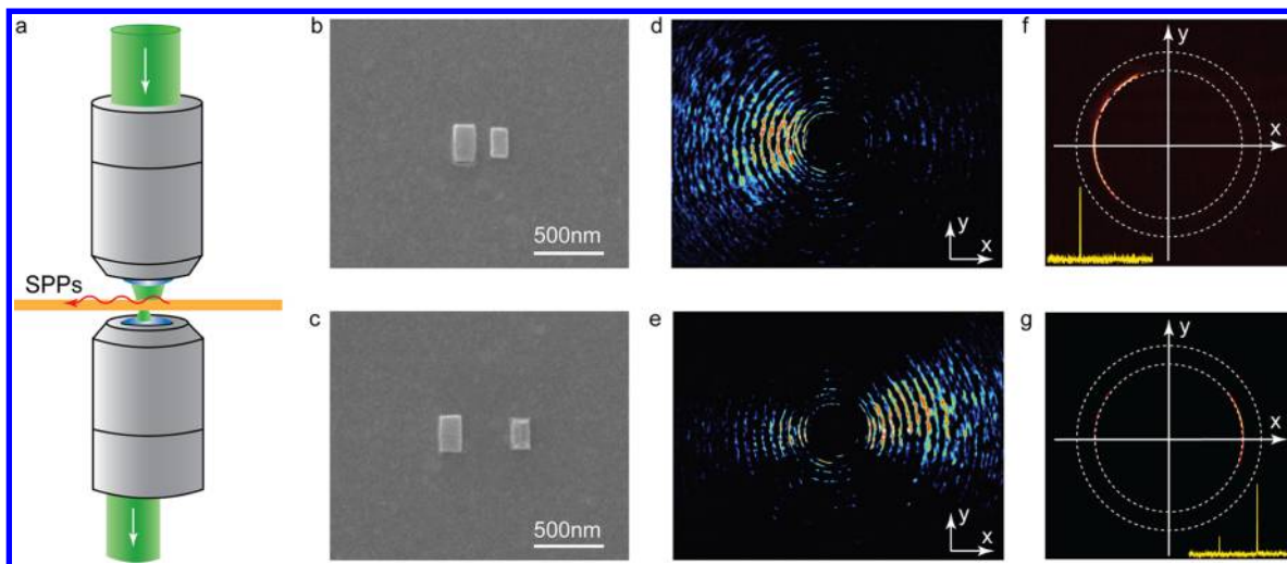
Figure 4. Experimental demonstration of the directional excitation of SPPs. (a) Schematic illustration of the experimental setup. (b, c) Scanning electron microscope (SEM) images of the fabricated nanoantenna sample. The distance between the two magnetic resonators is 300 and 600 nm, respectively. (d, e) Leakage radiation microscopy results for nanoantennas (b, c), respectively. The collected phase fronts of the SPPs launched at the air–gold interface are irrefutably directional and are remarkably in agreement with the theoretical simulation shown in Figure 3. (f, g) Respective Fourier plane of the images (d) and (e). The leakage radiation collected by the oil immersion objective clearly confirms the directionality of the SPP waves, which are emitted just above the critical angle (smaller dashed circle), as expected from the evanescent nature of SPPs. The yellow curves in the insets of (f, g) represent the line profile along the x -axis of the Fourier plane.
