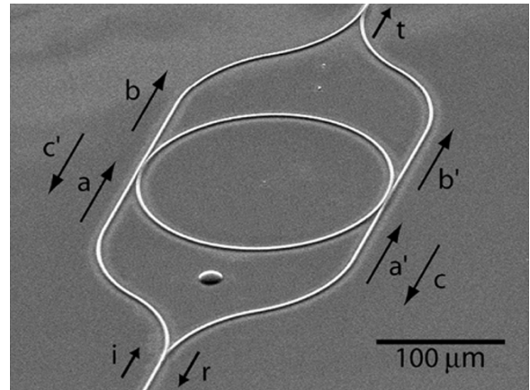
Fig. 1. Scanning electron microscope perspective image of a device similar to that measured here. The input, reflected, and transmitted signals are labeled i , r , and t , respectively. Two sets of fields, a , b , c and the corresponding primes obey (2) and (3).
