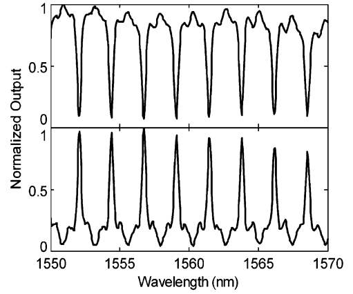
Fig. 3. Measurement results showing the normalized transmission (upper) and reflection (lower) signals. The extinction ratios for the nulls in the transmission signal are better than 10 dB.
