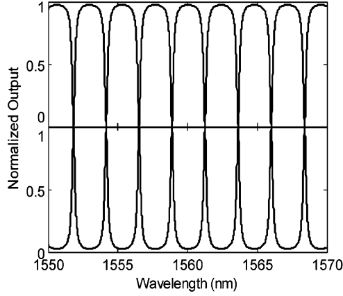
Fig. 2. Normalized transmission (upper) and reflection (lower) signals for the microring-based inline reflector. For the calculation, the microring radius is 108.25 \mu\text{m} , the effective refractive index is 1.515, t is 0.85, and the loss parameter \alpha is taken to be 1.
