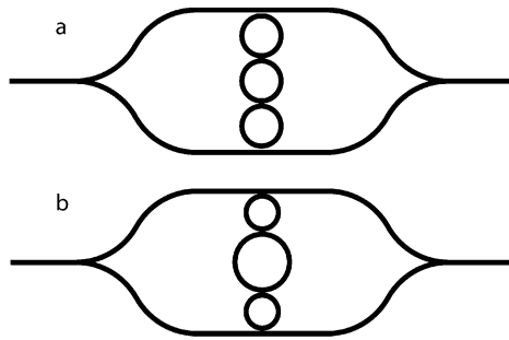
Fig. 4. (a) Reflector employing three microring resonators to exhibit a special spectral response, for instance, a wavelength-flattened reflection band. (b) Reflector employing the Vernier effect, with resonators of different radii.
