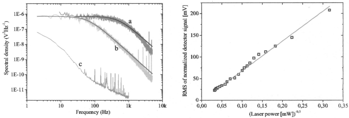
FIG. 3. (Left-hand side) Thermal noise spectra for 3180 nm bead (a) trapped at a laser power of 900 mW (corner frequency f_c = 502.9 Hz, force constant k = 94.7 pN/ \mu\text{m} ), (b) trapped at a laser power of 60 mW (corner frequency f_c = 63.1 Hz, force constant k = 11.9 pN/ \mu\text{m} ), (c) empty trap at a laser power of 60 mW. (Right-hand side) Linear dependency between rms value of the normalized detector signal (proportional to the displacement of the bead inside the trap) and the inverse square root of the laser power.
