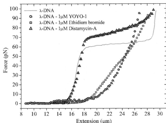
FIG. 5. Changes in the force response of \lambda -phage dsDNA in the presence of DNA binding agents. \lambda -phage dsDNA reference, YOYO-1 intercalated \lambda -DNA, EtBr intercalated \lambda -DNA, and \lambda -DNA complexed with Distamycin-A.
