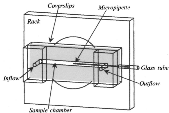
FIG. 2. The fluid chamber.
