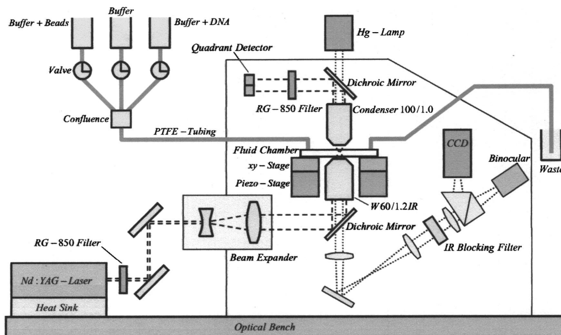
FIG. 1. Optical tweezers setup with integrated flow system.
