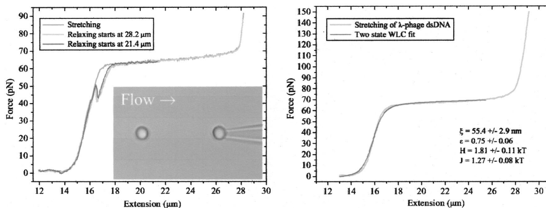
FIG. 4. (Left-hand side) Overstretching of \lambda -phage dsDNA in a force–extension/relaxation loop. Reproducible force hysteresis effects can be identified during relaxation. Inset: Single video frame obtained during the optical tweezers experiment. A bead ( 3.18 \mu\text{m} diameter) coated with streptavidin is held on a micropipette. A second bead (left-hand side) is trapped in the laser beam. A single biotinylated dsDNA molecule is attached to both streptavidin-coated spheres. (Right-hand side) two-state wormlike chain fit of the experimental data of free \lambda -phage dsDNA elasticity at the B – S transition and force–extension data of stretching dsDNA at higher laser power (900 mW) reveals high precision measurements and an extended force range up to 150 pN.
