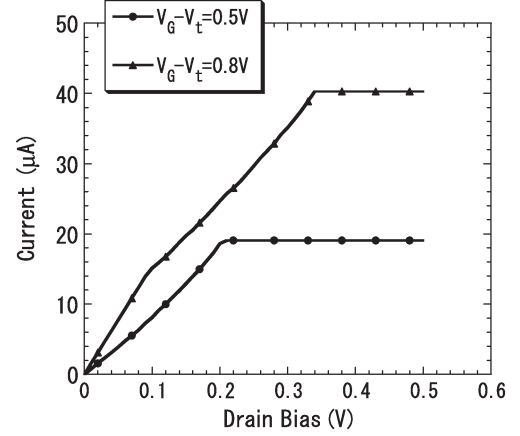
Fig. 5. I - V_D characteristics for a tentative simple subband structure at T = 0 . Parameters are m_0 = m_1 = 0.19 m , g_0 = g_1 = 1 , E_{00} = 0 , E_{10} = 0.16 eV, and C_G = 2.5 pF/cm. The solid circle (triangle) curve shows the case with the source Fermi level arrangement in Fig. 3(a) and (b).
