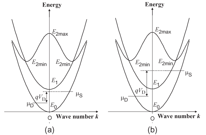
Fig. 3. Example of the E - k relation of the nanowire's subband. (a) Case where the lowest subband is mainly populated. (b) Case where the lowest two subbands are mainly populated.
