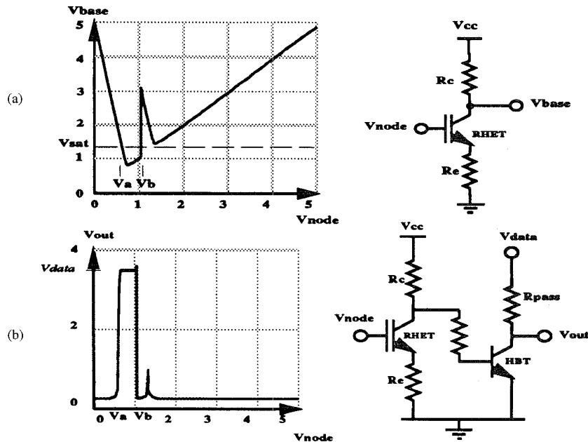
Fig. 6. (a) RHET/RTBT in inverter circuit configuration. (b) A literal-pass gate.
