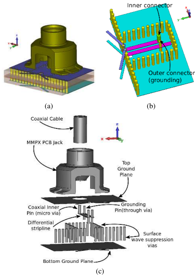
Fig. 14. (a) 3D view of the antenna with the MMPX connector and feeding structure and (b) view of the internal feeding structure, and (c) Exploded view of the connector and feeding structure.
