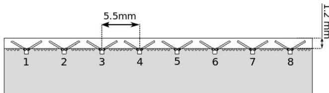
Fig. 8. The geometry of the proposed antenna array.
