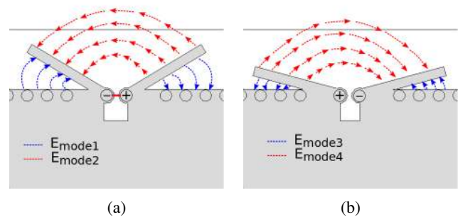
Fig. 2. Electric fields of the proposed antenna's modes in (a) top view and (b) bottom view.
