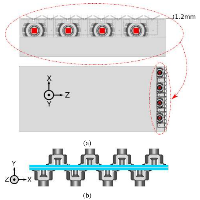
Fig. 16. Geometry of the phased antenna array with connectors (a) top view and (b) side view.
