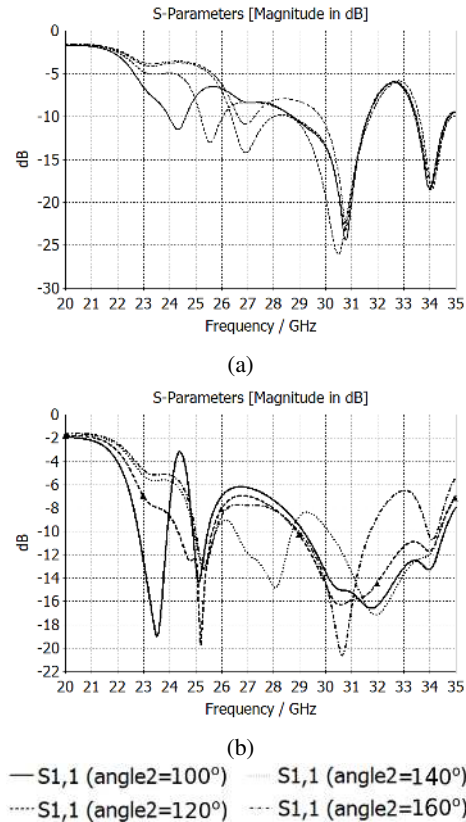
Fig. 4. Parametric sweep of (a) Ang1 and (b) Ang2.
