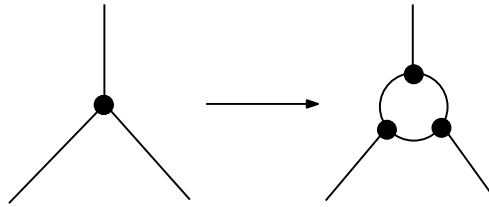
Figure 12: How to blow up a vertex
