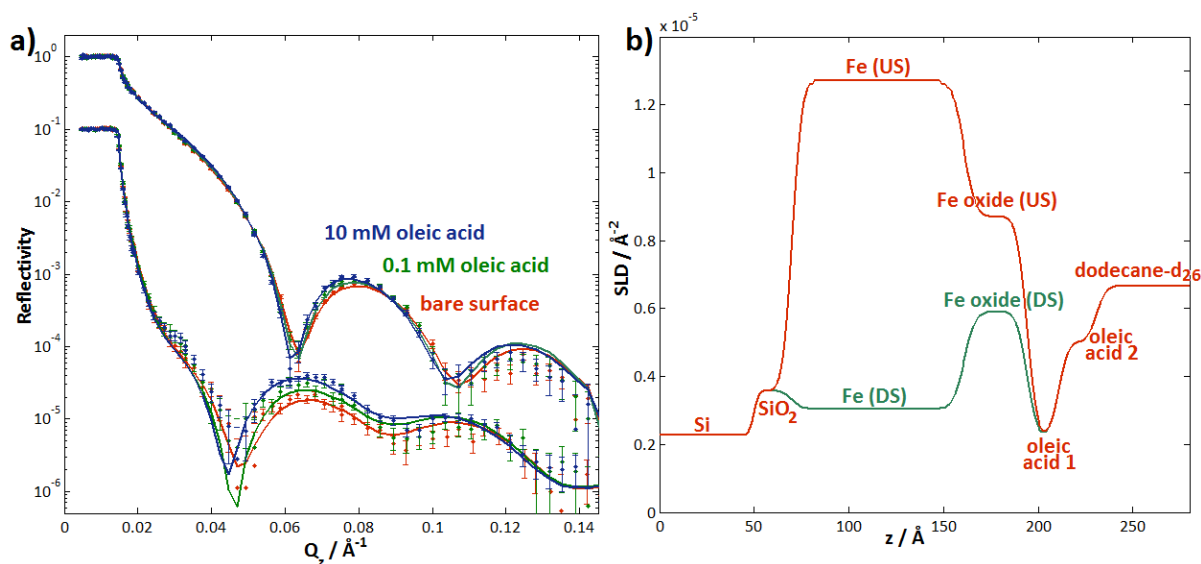
Figure 4. a) PNR profiles of the iron oxide/oleic acid/dodecane- \text{d}_{26} system, with just the lowest and highest concentrations shown, as marked. (Data shown as points with fits as solid lines. The down-spin data are shown offset vertically by a factor of 10 for clarity.) b) Fitted SLD profiles for the 0.01 M oleic acid system, showing the two acid layers (US = up-spin; DS = down-spin).
