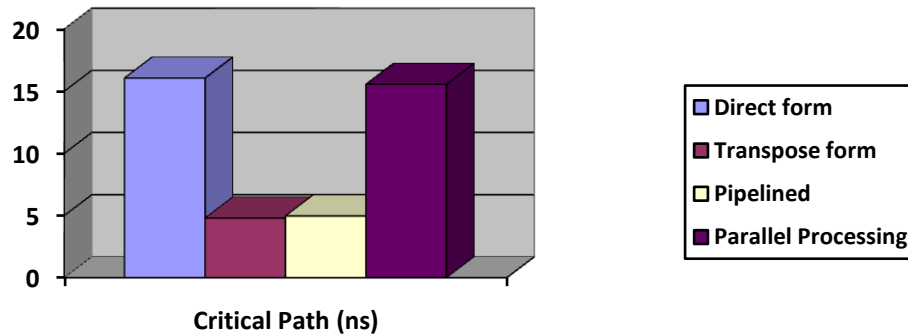
Figure8 Minimum Period(ns)
