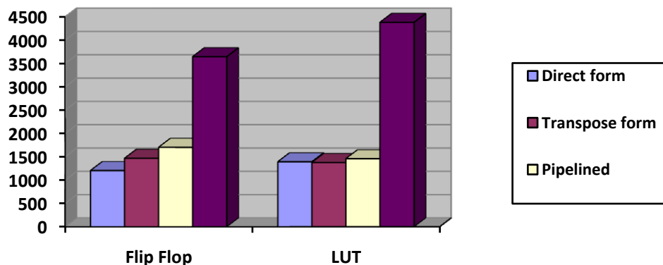
Figure7 Resource utilization
