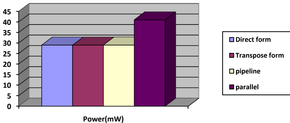
Figure10 Power Consumption
