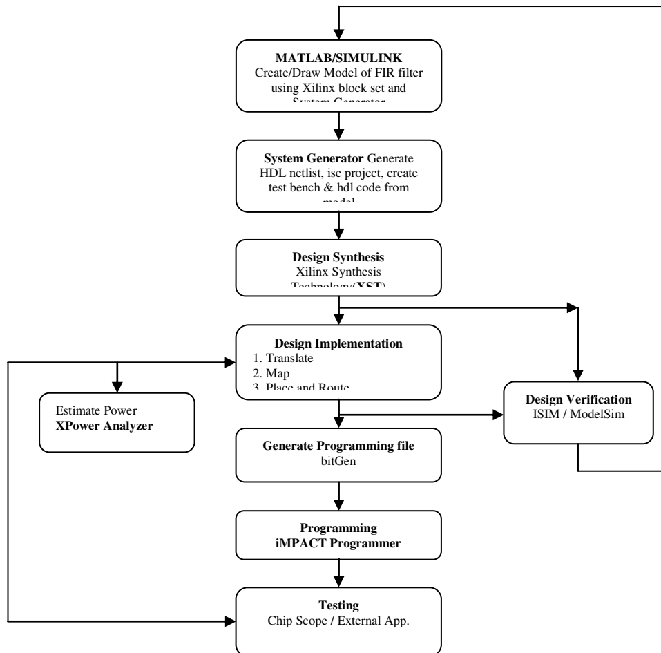
Figure3. Design flow of FPGA
