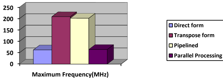
Figure9 Maximum Frequency (MHz)
