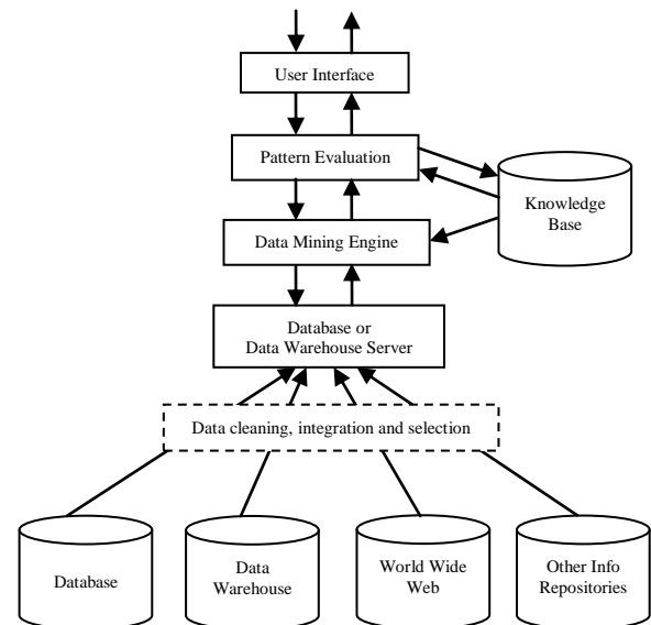
Fig 1: Architecture of a Typical Data Mining System
