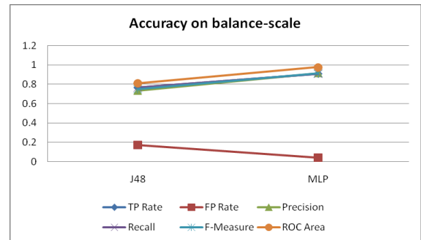
Fig 3: Accuracy chart on balance-scale
