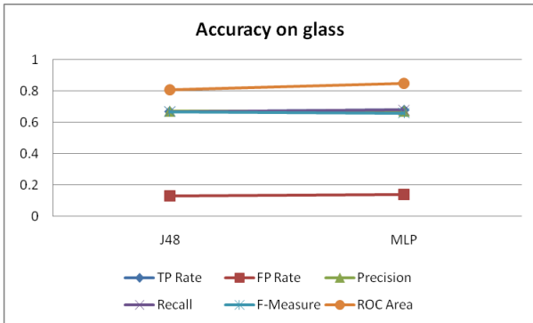
Fig 5: Accuracy chart on glass
