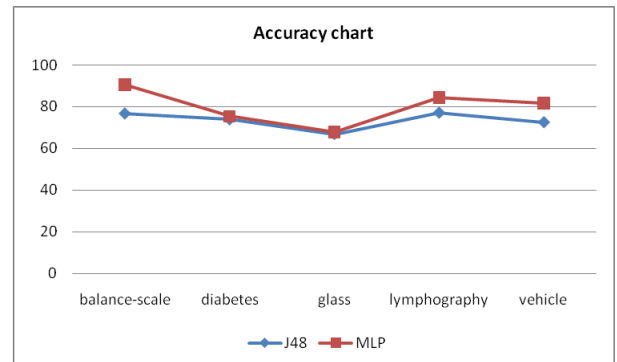
Fig 8: Accuracy chart of J48 and MLP
