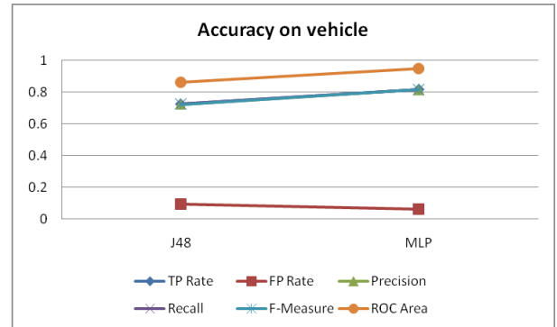
Fig 7: Accuracy chart on vehicle
