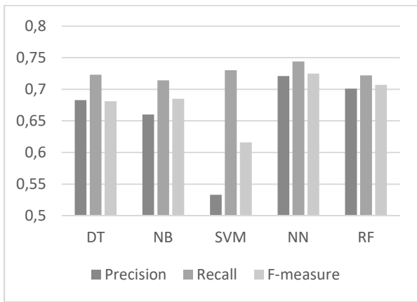
Fig. 1 Comparison of cross-validation approach among the five techniques
