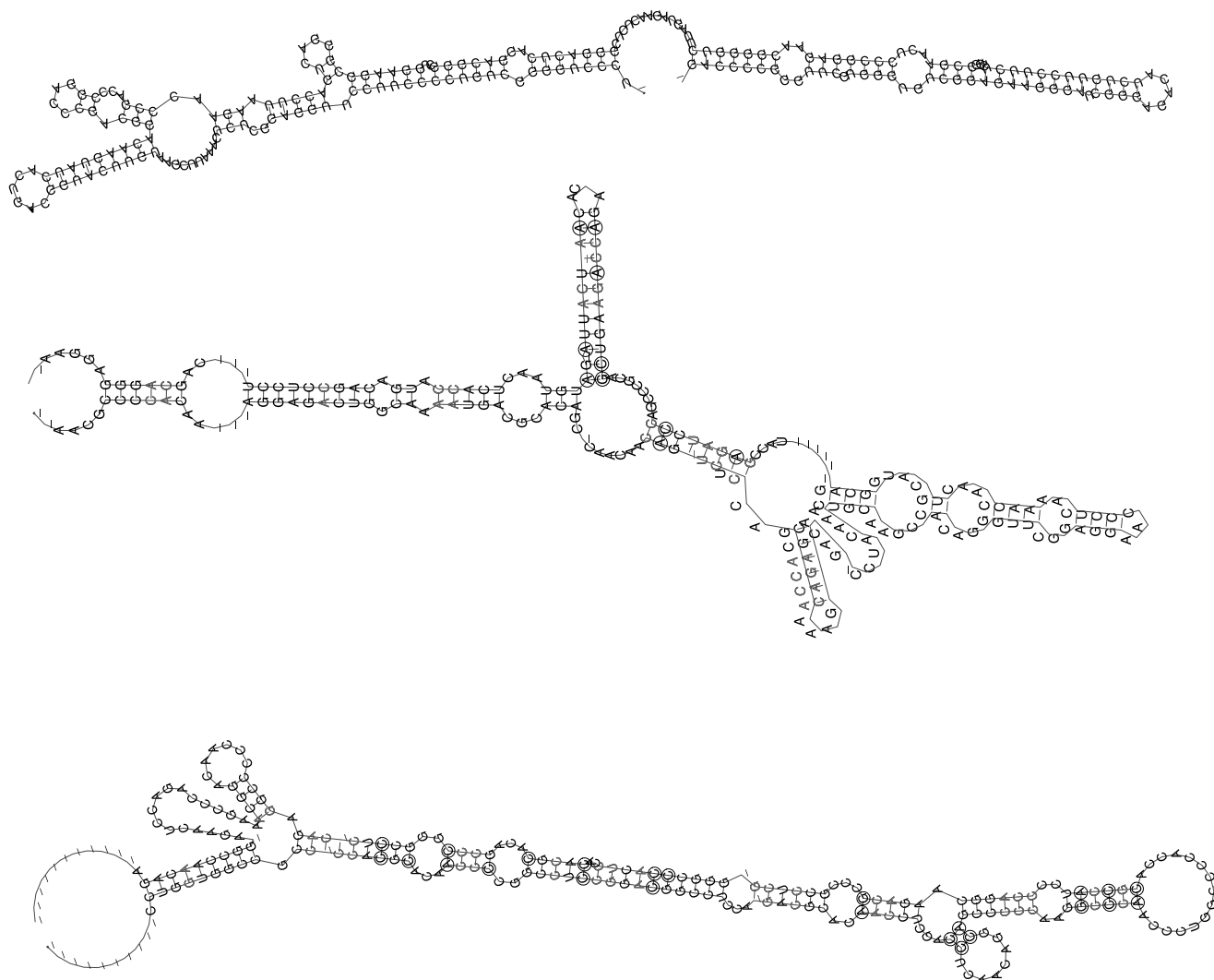
Figure 2 Example of secondary structures of three candidates for novel primate-specific non-protein-coding RNAs as predicted by program RNAZ. The genomic coordinates (NCBI build 34) of the three TARs are chromosome 2:10,415,689–10,415,908; chromosomes 11: 11,3423,510–113,423,729; and chromosome 7:56,614,161–56,614,382.
