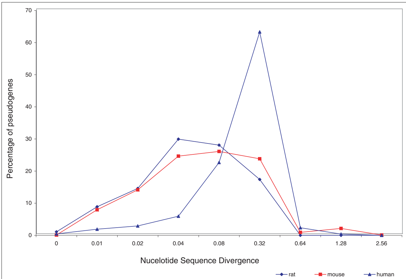
Figure 4 Processed pseudogenes grouped according to their nucleotide sequence divergence from the parent RP protein. The distances have been calculated using MEGA [28]. The distance is a measure of the number of nucleotide substitutions per site. For mouse and rat, the distances have been scaled by decreasing it by a factor of three based on the reported observation that a threefold-higher rate of base substitution in neutral DNA is found along the rodent lineage when compared with the human lineage [20].
