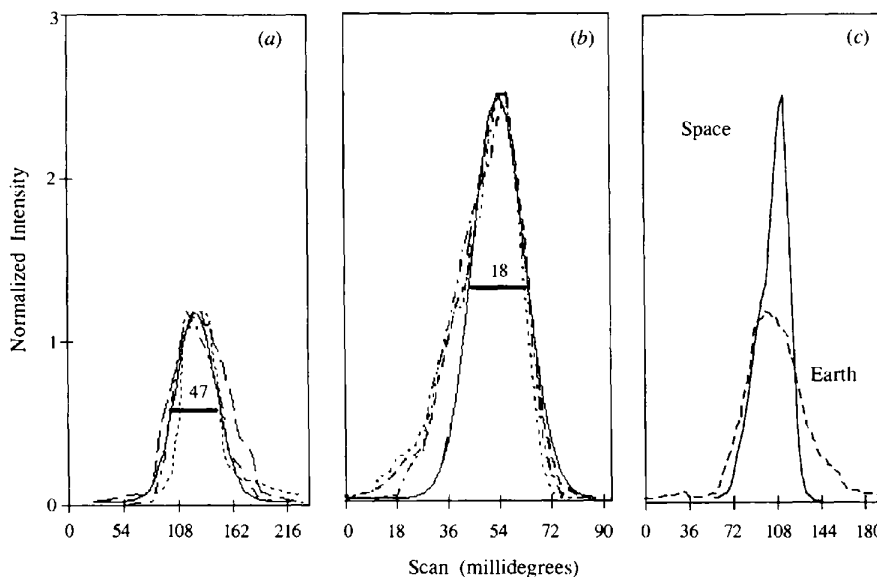
Fig. 5. Profiles of three representative reflections, (17, \bar{1}, 23) , (\bar{2}, 12, 12) and (16, \bar{10}, 5) , at 4 Å were evaluated from (a) earth- and (b) space-grown thaumatin crystals from the LMS experiment. Reflections were obtained in the vertical diffraction plane such that the rotation axis was horizontal and perpendicular to the X-ray beam. Each set of reflection profiles for space- and earth-grown crystals were averaged and Gaussian fits of the sets of profiles were calculated (solid lines). The Gaussian plots were fitted to the principle peaks, for which the FWHM values were obtained. Only the principle peak is considered to represent the actual mosaicity profile for space-grown crystals. The FWHM of a Gaussian fit for each profile was measured and its value deconvoluted out by the value of the instrument resolution function, IRF (0.15 mrad or 0.009°). FWHM values are indicated by short horizontal lines in the profiles; they show that the space-grown crystals are about two and a half times less mosaic than the earth-grown crystals. The intensities shown are normalized and the actual peak intensities were measured to 250 000 counts per 0.1 s for the space-grown crystal. In contrast, the spot intensities corresponding to the same reflections for the earth-grown crystal were approximately two times less. Part (c) shows a relative comparison of the averaged mosaicity profiles for an earth- and a space-grown crystal for the same reflections.
