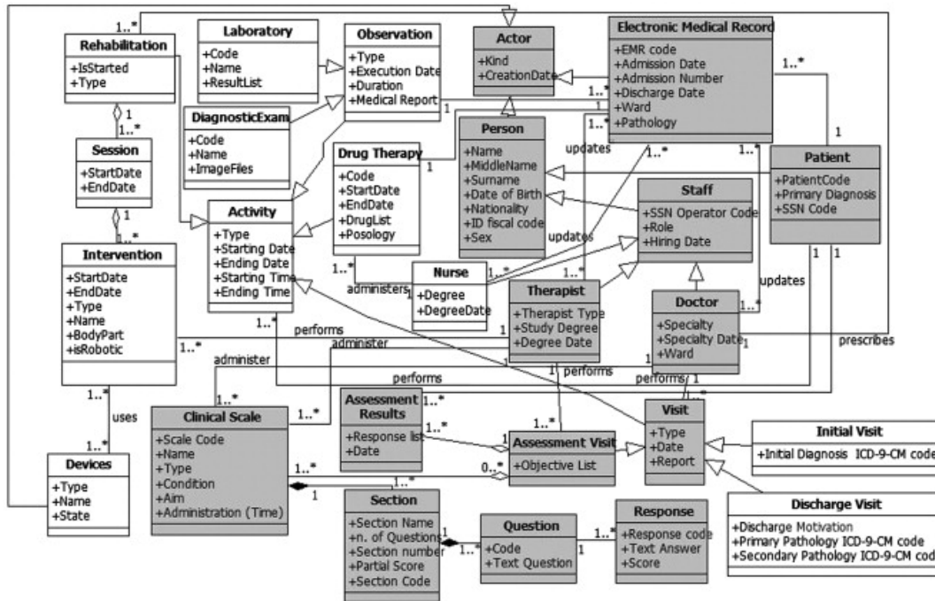
Figure 5. UML process modeling - class diagram of the post stroke rehabilitation process. Source: Ferrante et al. (2013).
