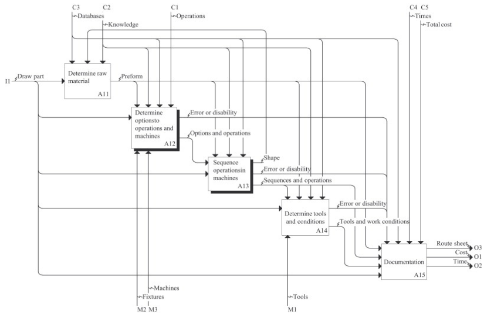
Figure 10. Process planning level in the IDEF model. Source: Ciurana et al. (2008).
