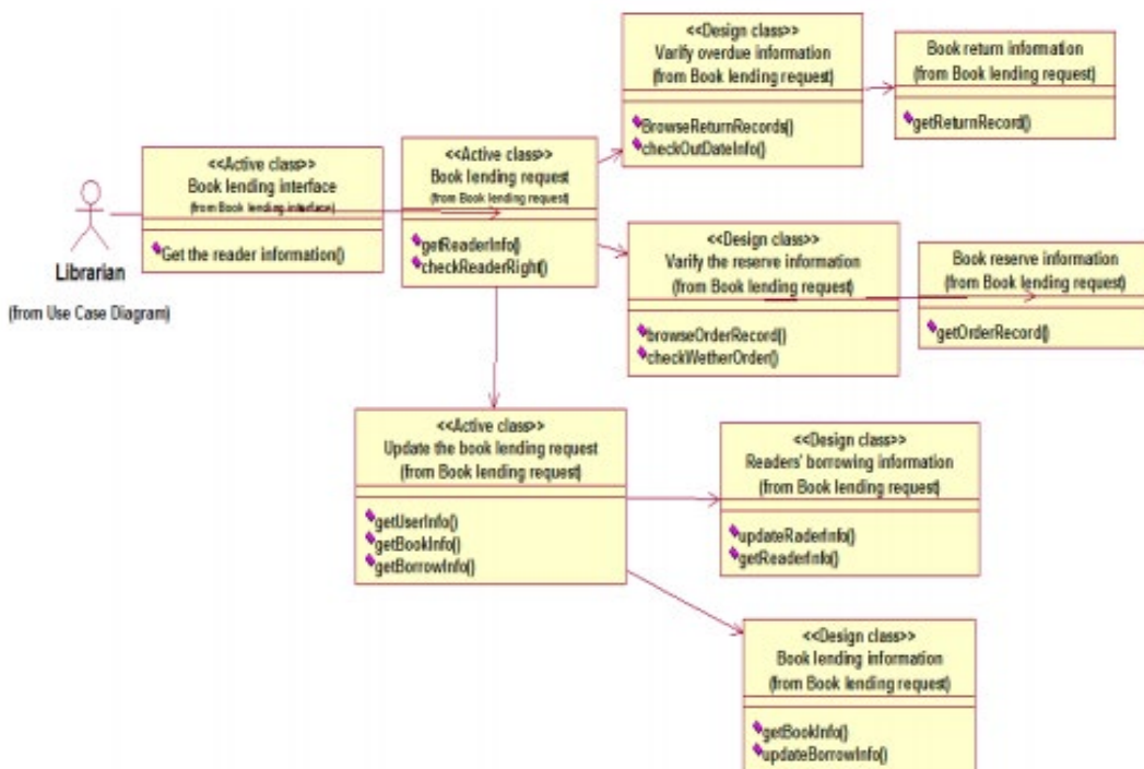
Figure 6. Diagram design classes of the management book loans. Source: Zheng et al. (2014).
