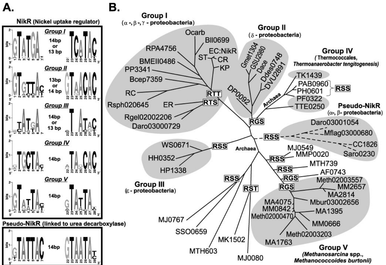
FIG. 1. Conservation of the NikR regulon in bacteria and archaea. (A) Sequence logos for the predicted NikR-binding signals in various taxonomic groups. (B) Maximum likelihood phylogenetic tree of the NikR proteins. All NikR-binding sites identified in the genomes that encode NikR from a certain group (marked by background gray) were used for construction of the sequence logo for the corresponding group. Candidate NikR-binding sites were not identified in only a few archaeal genomes encoding NikR (unmarked proteins on the phylogenetic tree). Three surface residues of the N-terminal beta sheets involved in DNA recognition are shown in boxes.
