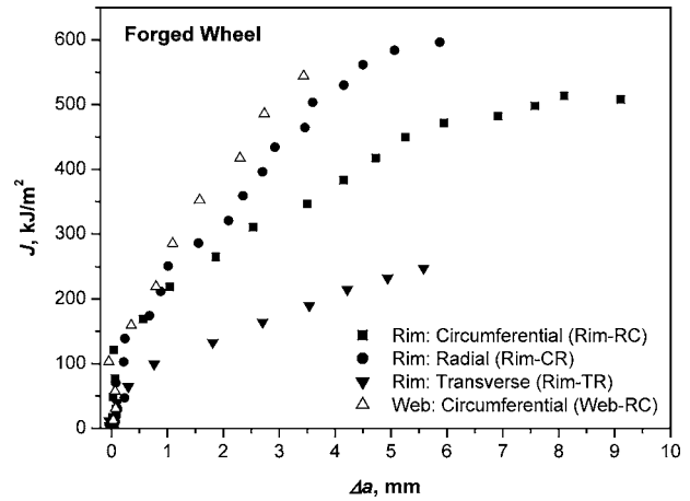
Fig. 16 J - R curves obtained from specimens of the forged rail wheel.
