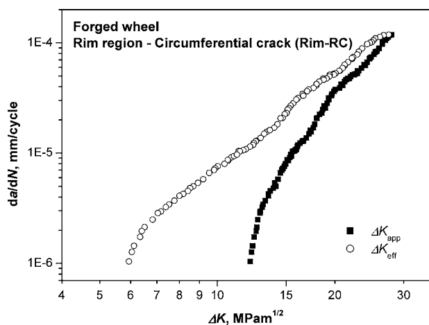
Fig. 9 Fatigue crack growth resistance of forged material from rim region with circumferential crack characterised by applied and effective \Delta K .
