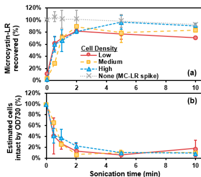
Figure 1. (a) Microcystin-LR (MC-LR) recovery (%) and (b) estimated cells remaining intact (by optical density at 730 nm, OD730) (%) versus sonication time (minutes). Error bars represent standard deviation from duplicate experiments. Data are shown for low ( \sim 10^5 cells/mL, red circles), medium ( \sim 10^6 cells/mL, yellow squares), and high ( \sim 10^7 cells/mL, blue triangles) density suspensions of laboratory-cultured M. aeruginosa in phosphate buffer. The MC-LR-spiked control solution (with no cells) is represented by the grey dotted line.
