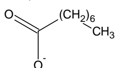
1 N,N-dimethylethanolammonium octanoate
