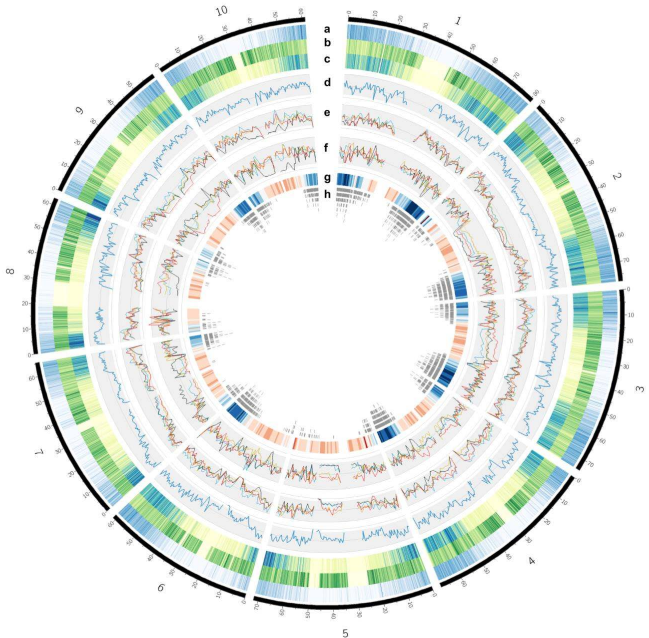
Figure 3. Genomic landscape of sorghum. a , Gene density heatmap. b , SNP density. c , Indel density. d , rho ( \rho ) population recombination rates were calculated using FASTPRR in 500kb windows. e , Nucleotide diversity ( \pi ) in 1Mb windows for each sorghum race, the color codes are the same as used in Figure 1A, (red=kafir, blue=caudatum, yellow=durra, dark green=guinea). f , Tajima's D for each sorghum race. g , Average GERP score per 1Mb window, with a divergent red-blue scale where blue represents high GERP score. h , Genomic distribution of sorghum non-fractionated genes.
