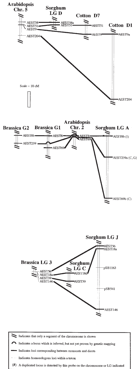
Figure 3. Examples of Colinearity of Monocot and Dicot Genes. Arabidopsis cDNAs that show DNA sequence conservation (BLASTx > 150) with genes from monocots or more distant taxa were used to
