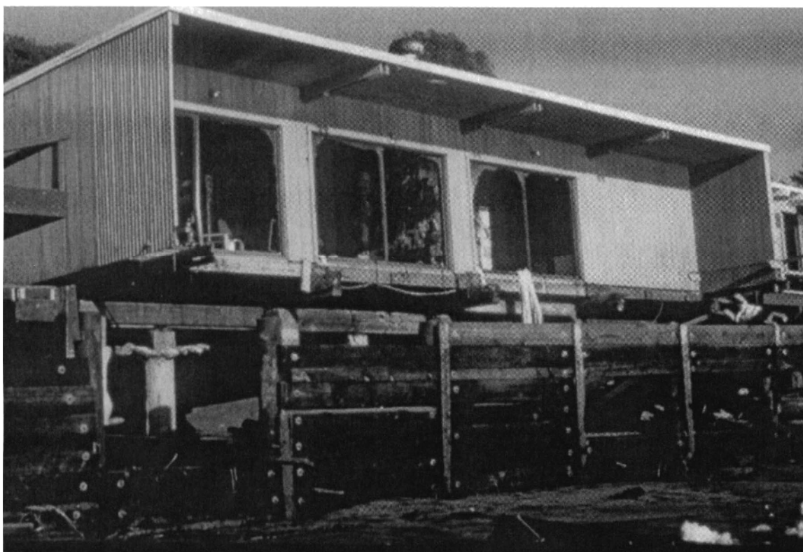
Figure 2. Damage to a house and timber seawall along Beach Drive in northern Monterey Bay resulting from the storms of early 1983. The seawall was battered and breached by waves and debris, allowing over 2 m of fill behind the wall to be scoured, undercutting the structure and threatening the structural support system.
