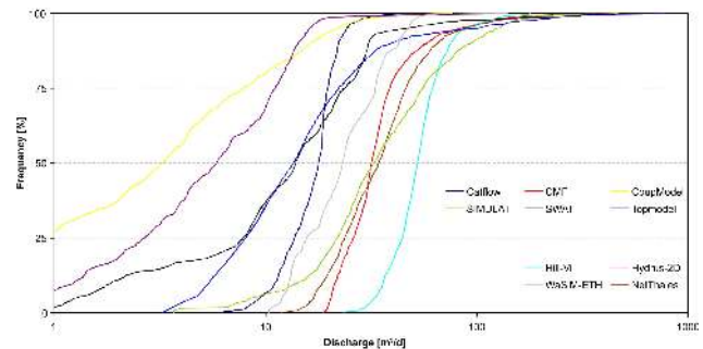
Fig. 5. Discharge-frequency relationship of the ten predictions.
