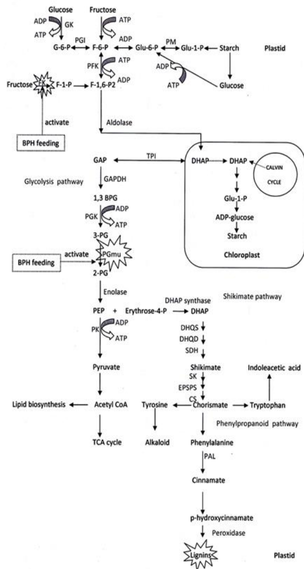
Fig 2. The activation of fructokinase (FK, EC 2.7.1.4) and phosphoglyceratemutase (PGmutase, EC 2.7.5.3) in fructose metabolism and glycolysis pathway connect to the tricarboxylic acid (TCA), Shikimate and phenylpropanoid pathway. The lignin is the end product of integrated pathway in current studies. The other related enzyme in glycolysis pathway were shown following: 6-Phosphofructokinase (PFK, EC 2.7.1.11), Phosphoglucomutase (PM, EC 2.7.5.1), Phosphoglucose isomerase (PGI, EC 5.3.1.9), Aldolase (EC 4.1.2.13), Triosephosphate isomerase, (TPI, EC 5.3.1.1), glyceraldehyde-3-phosphate dehydrogenase (GAPDH, EC 1.2.1.12), phosphoglycerate kinase (PKG, EC 2.7.2.3), Enolase (EC 4.2.1.11), Pyruvate kinase (PK, EC 2.7.1.40), In shikimate pathway; Dehydroquinase (DHQS, EC 4.2.3.4), Dehydroquinase (DHQD, EC 4.2.1.10), Shikimate dehydrogenase (SDH, EC 1.1.1.282), Shikimate kinase (SK, EC 2.7.1.71), 5-Enolpyruvylshikimate 3-Phosphate synthase (EPSPS, EC 2.5.1.19), Chorismate synthase (CS, EC 4.2.3.5). Finally, enzyme in Phenylpropanoid pathway; Phenylalanine ammonia lyase (PAL, EC EC 4.3.1.24). and peroxidase. Adapted from Mukutu and Nose (2012).
