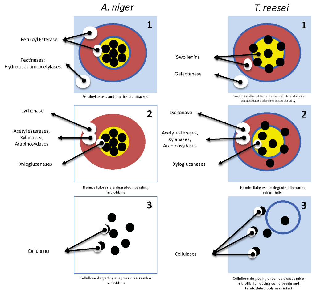
Fig 6. Schematic representation of hypothetical modes of attack of the enzyme complexes produced by A. niger (left) and T. reesei (right). One cell wall architectural unit of sugarcane (De Souza et al., 2013) is represented. Light blue: pectins; dark blue: feruloyl esters; red: hemicelluloses—beta-glucan and arabinoxylan; yellow: xyloglucan; black: cellulose microfibrils. Cell wall degradation is schematically represented in three steps for each fungi attack so as to compare the two different strategies hypothesized in this work. Whereas A. niger degrades cell wall components of different classes with approximately the same intensity, including action on feruloyl esters, pectins, hemicelluloses and cellulose, T. reesei maximizes penetration into the cell wall matrix, lacking feruloyl esterases, having limited action on pectins, but disassembling more efficiently the cellulose-xyloglucan network and attacking mainly the cellulose microfibrils.
