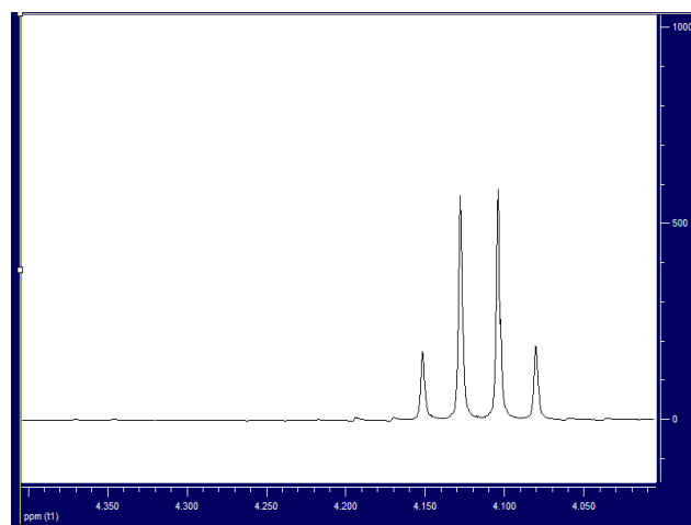
Fig. 2. Quartet characterizing peaks of palmitate.
