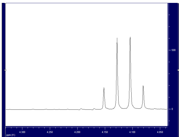
Fig. 3. Quartet characterizing peaks of stearate.
