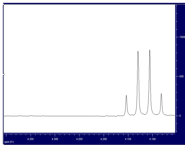
Fig. 3. Quartet characterizing peaks of oleate.
