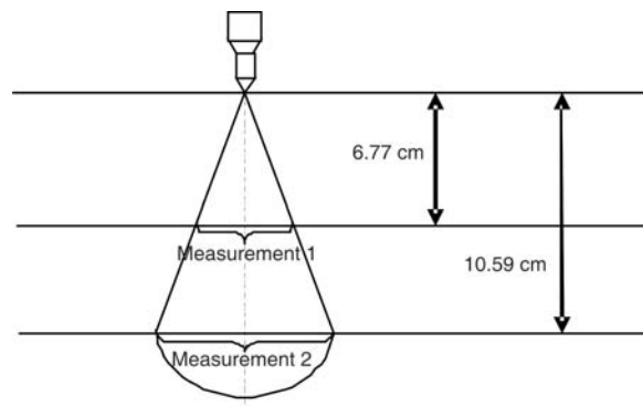
Figure 6. Spray pattern and measurement locations
