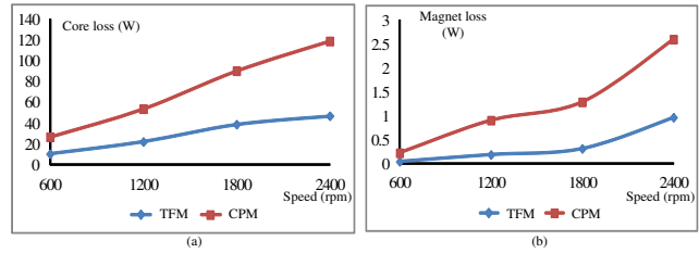
Fig. 8. No-load loss of TFM and CPM: (a) core losses, and (b) magnet eddy current loss.
