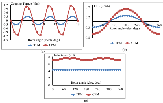
Fig. 7. 3D FEA results of CPM and TFM: (a) cogging torque, (b) no-load flux per turn of stator coil, and (c) inductance of per turn of stator coil.
