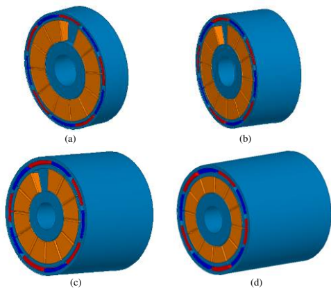
Fig. 11. Topology of outer rotor RFM with different ratio of axial length to outer radius, (a) 0.5, (b) 1, (c) 1.5 and (d) 2
