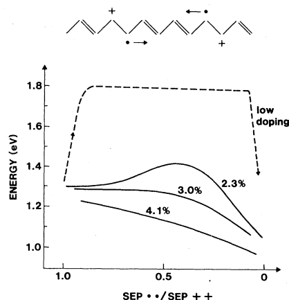
FIG. 4. Interaction between two radical cations (or polarons) in polyacetylene. The horizontal axis is the ratio of the radical separations to the charge separations so that the right extreme of the figure represents the formation of two charged solitons from two polarons. Doping levels as mole per cent are indicated.
