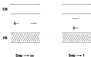
FIG. 3. Interaction of charged and neutral soliton in polyacetylene. States appear at midgap for infinite separation but interact and split as indicated when the separation approaches one bond (polaron formation).
