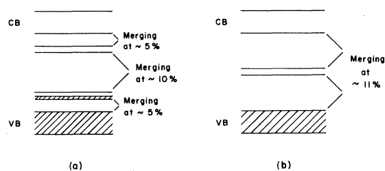
FIG. 5. Band-structure scheme at intermediate doping for a lattice of polarons (a) and a lattice of charged solitons (b). At higher doping levels, bands in the gap broaden and this leads in our model for case (a) to the merging of the bonding (antibonding) band with the valence (conduction) band at \sim 5\% doping level while the bonding and antibonding bands merge at \sim 10\% doping. For case (b), the soliton band merges with the valence and conduction bands at \sim 11\% doping, in agreement with Mele and Rice calculations (Ref. 44). Following these authors, inclusion of interchain coupling could reduce the doping level where merging occurs to below 5\% where it is observed experimentally.
