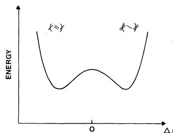
FIG. 1. Sketch of potential energy curve for trans polyacetylene showing two energetically equivalent structures.
