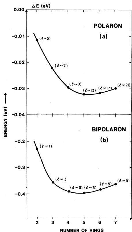
FIG. 11. Energy gain with respect to vertical ionization processes obtained in polyparaphenylene through the formation of a polaron for a singly charged defect (a) and of a bipolaron for a doubly charged defect (b), as a function of the extension of the defect, in number of rings N . For each N value, the optimal l value is shown in parentheses.
