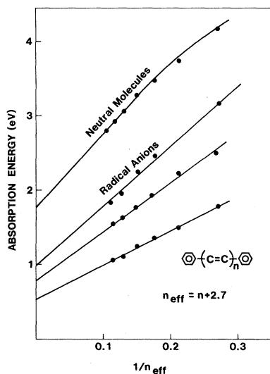
FIG. 7. Optical absorption energy vs the reciprocal of the "effective" number of double bonds for diphenyl polyenes (neutral molecules and radical anions). The solid line through the neutral molecule data represents data for polyenes (with extrapolation) taken from the literature (Ref. 33).
