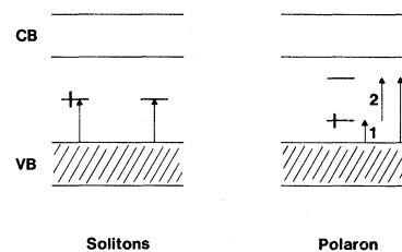
FIG. 6. Schematic representation of doping-induced optical transition in polyacetylene for solitons and polarons.
