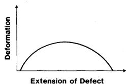
FIG. 10. Deformation model for polyparaphenyrene chain based on product of hyperbolic tangent functions.
