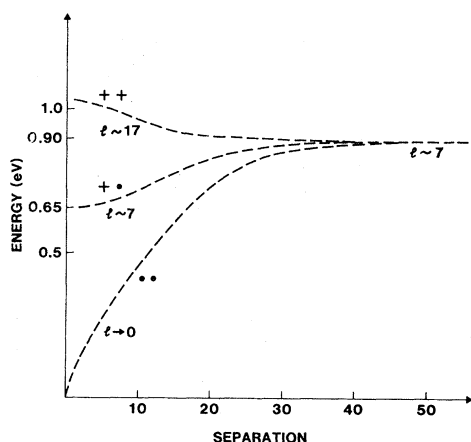
FIG. 2. Energetics of separation of two defects on polyacetylene chain with “..” indicating two radicals (neutral solitons), “++” indicating two cations (charged solitons) and “+.” indicating a radical cation (or polaron for small separations). The quantity l defines the extent of the chain deformation due to the defect. The units for the abscissa and l are number of carbon atoms.
