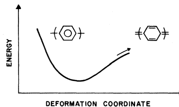
FIG. 8. Sketch of potential energy curve for polyparaphenylene showing energetically inequivalent structures.
