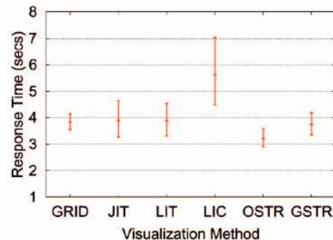
Fig. 8. Mean time to perform the advection task in seconds. The error bars shown are 95 percent inferential confidence intervals; nonoverlapping bars indicate a statistically significant difference between those means. The graph indicates that users took significantly longer to perform the advection task using LIC than using OSTR, GSTR, and GRID.
