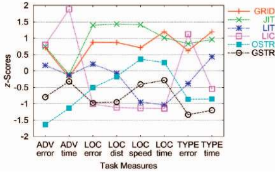
Fig. 15. z-scores for each visualization method calculated for each task measure. The z-scores represent the difference between the mean performance for a method and the mean performance for all methods for each task. This difference is divided by the standard deviation of the mean performance for each task to provide a measure with units of standard deviation. This transformation allows comparisons between the relative patterns of performance of each method across the task measures. The categories along the x-axis represent the task measures: ADV (advection) error and time; LOC (critical point location) counting error, distance error, flow speed error, and time; and TYPE (critical point type identification) error and time. Scores above zero indicate more error or slower performance on the task, while scores below zero indicate less error or faster performance.
