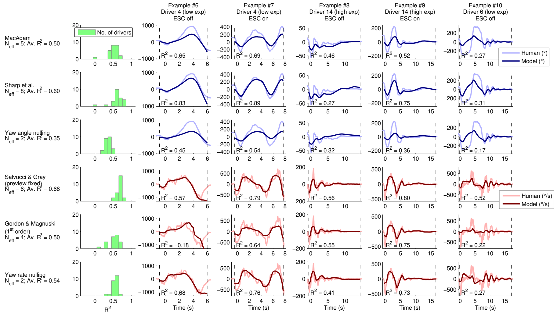
Figure 7. Stabilization steering. Distributions of average model performance (leftmost panels) and comparison of human and model steering in five example recorded scenarios, for six of the tested models. Besides including both novices and experienced drivers, driving with and without ESC, the example recordings have been chosen to illustrate typical model performance across various steering behaviours, and to highlight strengths and weaknesses of the different models. Note that the top three rows show models controlling steering angle ( \delta ), whereas the bottom three show models controlling steering rate ( \dot{\delta} ), thus deviating somewhat from the order of model presentation in Sect. 2.2.
