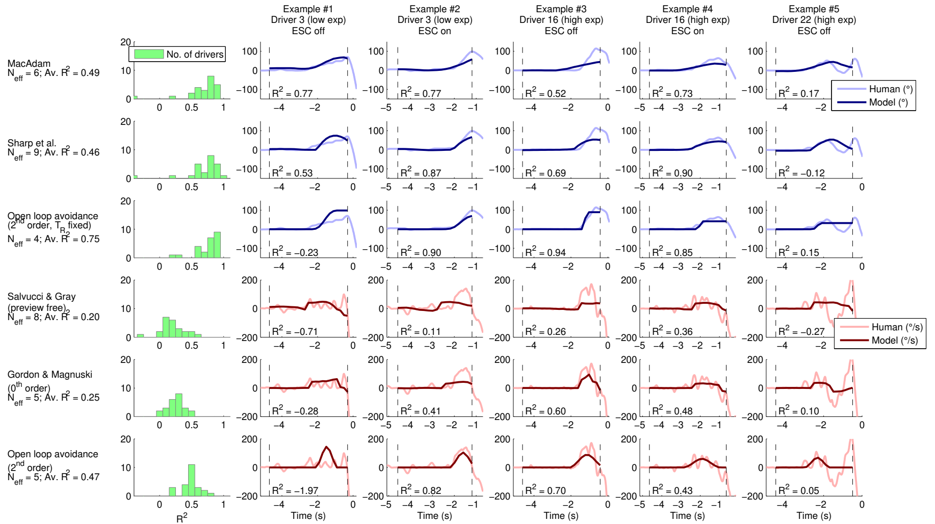
Figure 6. Collision avoidance steering. Distributions of average model performance (leftmost panels) and comparison of human and model steering in five example recorded scenarios, for six of the tested models. Besides including both novices and experienced drivers, driving with and without ESC, the example recordings have been chosen to illustrate typical model performance across various steering behaviours, and to highlight strengths and weaknesses of the different models. Note that the top three rows show models controlling steering angle ( \delta ), whereas the bottom three show models controlling steering rate ( \dot{\delta} ), thus deviating somewhat from the order of model presentation in Sect. 2.2.
