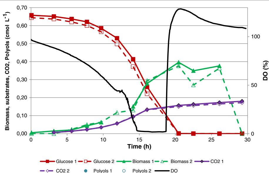
Figure 1 Batch cultivation of Y. lipolytica with 20 g L -1 glucose (0.65 \text{cmol L}^{-1} ) showing substrate, biomass and product concentration as a function of time.
