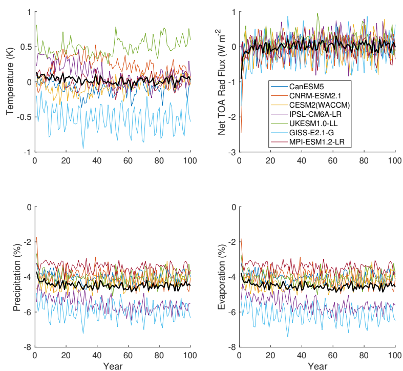
Figure 1. Temperature (top left; K), net top-of-atmosphere radiative flux (top right; \text{W m}^{-2} ), precipitation (bottom left; %), and evaporation (bottom right; %) change in G1 CMIP6 compared to piControl over 100 years of simulation. Thin colored lines are individual models, and thick black lines are ensemble means.
