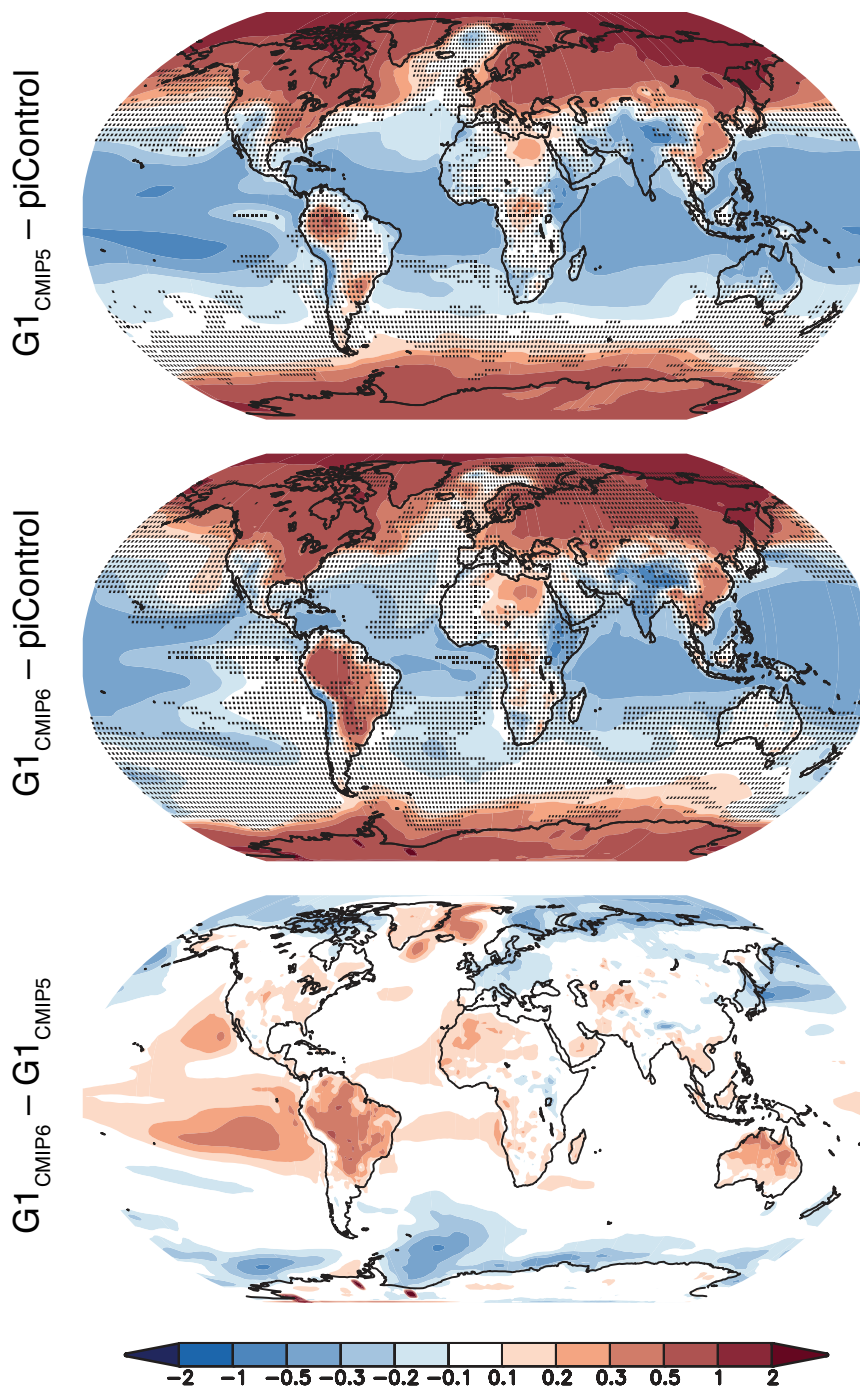
Figure 8. Ensemble average temperature changes (K) for G1 (as compared to the preindustrial control) for CMIP5 (top) and CMIP6 (middle), as well as the difference ( G1_{\text{CMIP6}} minus G1_{\text{CMIP5}} , bottom panel). In the top two panels, stippling indicates regions where fewer than 75% of the models in their respective ensembles agree on the sign of the response.
