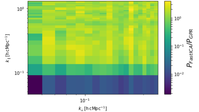
(c) Looking at the 2D cylindrical power spectrum for ratio between FastICA's and GPR's foreground removal residual of the LOFAR 10 Nights Data.
