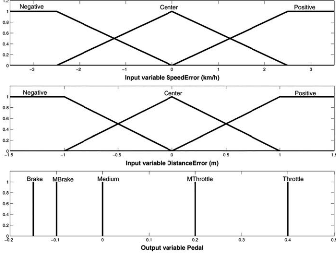
Fig. 3. Membership functions.
