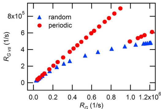
Fig. 3. (Color online) Rate of VALID STARTs on the gate R_{G\ vs} is plotted versus STARTs R_G . Circles are for a periodic train of STARTs, while triangles are for a random stream of STARTs from the downconversion source.
