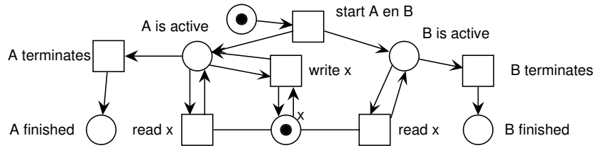
Fig. 11. Example of concurrent access to shared data. Activities A and B both access data item x
