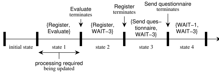
Fig. 4. Example run in requirements-level semantics
