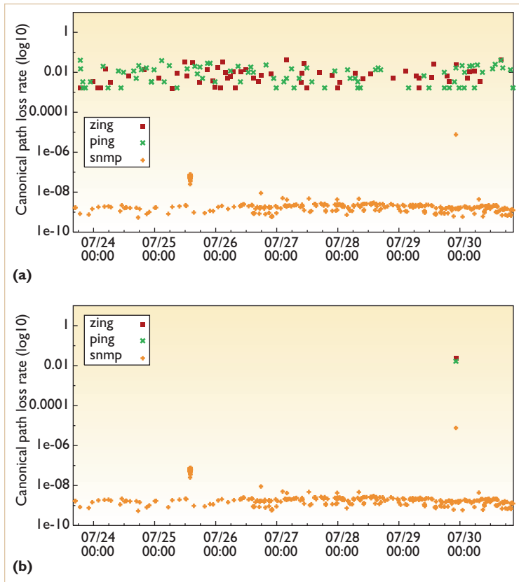
Figure 1. Loss rates. We compared loss rates on the Indianapolis, Indiana, to Los Angeles, California, canonical path for a 20-Hz probe rate. Simple Network Measurement Protocol (SNMP) measurements were identical for each data set, but filtered data sets contained only active probe events when we measured a loss event at a router in the corresponding sample interval.
