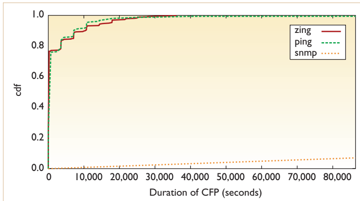
Figure 4. Change-free periods on the canonical path. During the 20-Hz probe period, the cumulative distributions of change-free periods (CFPs) for all paths don't match exactly, indicating that probe-based CFP marginals are not good approximations for router-based ones that suggest much more steady loss rates.
