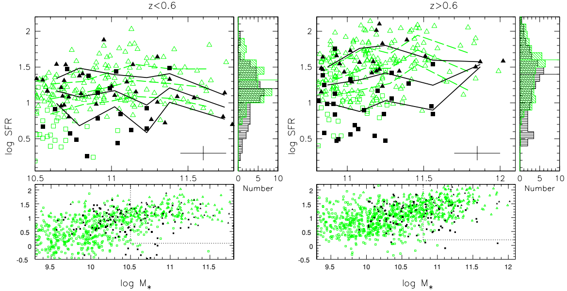
Figure 1. SFR– M_* relation of cluster and field galaxies at z < 0.6 (left panel) and z > 0.6 (right panel). Only 24 \mu\text{m} +BEL galaxies are plotted. Upper left window: only data points above the completeness limits. Bottom window: all galaxies. Black filled symbols: cluster galaxies (EDiCS). Green empty symbols: field galaxies (AEGIS). Triangles: combined SFRs from MIPS 24 \mu\text{m} and emission lines. Squares: [O II] dust-corrected SFRs. In the upper window, lines represent the median and the 25 and 75 percentiles for the clusters (solid black) and field (dashed green). Typical EDiCS error bars are in the bottom right. In the bottom window, lines show the mass and SFR limits. Upper right window: SFR distribution of galaxies above the completeness limits, selecting the same mass distribution in clusters and field, for the average of the 1000 simulations. The number of field galaxies is normalized to the number of cluster galaxies. Black slanted histogram: AEGIS. Black (EDiCS) and green (AEGIS) solid lines are the mean values of the distributions.
