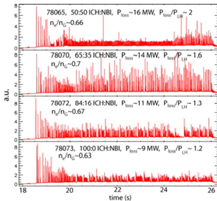
Figure 2a: Combined heating H-modes (IC and NBI) with varying proportion of IC power (from 50 to 100% IC), and varying total input power (from ~16 MW to ~9 MW). At each level of power, apart from the 9 MW, the corresponding comparison H-mode with NBI only is shown in Fig. 2b.
