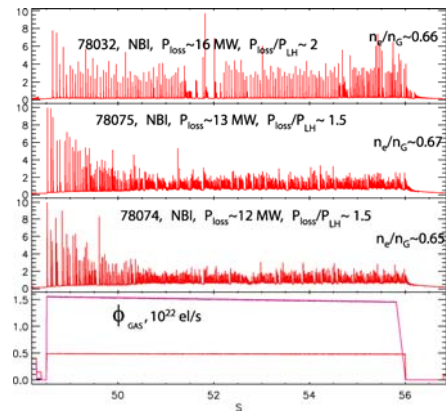
Figure 2b: H-modes heated only by NBI with varying total input power (from ~16 MW to ~12 MW). At each level of power the corresponding comparison H-mode with NB+IC only is shown in Fig. 2a. The Figure also shows that the two levels fuelling flux \phi_{\text{gas}} the lower one for the H-mode at 16 MW, the highest one for the others as well as for the comparison H-modes in Fig. 2a.
