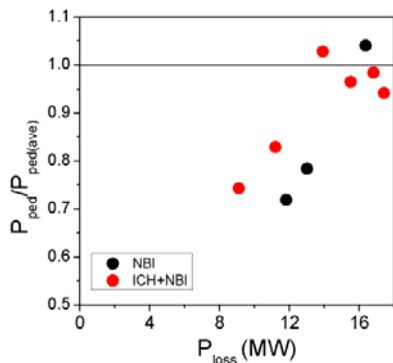
Figure 10: Pedestal pressure normalised to the constant pressure value of Fig. 8, showing that the decrease in pedestal pressure is due to the decrease in input power
