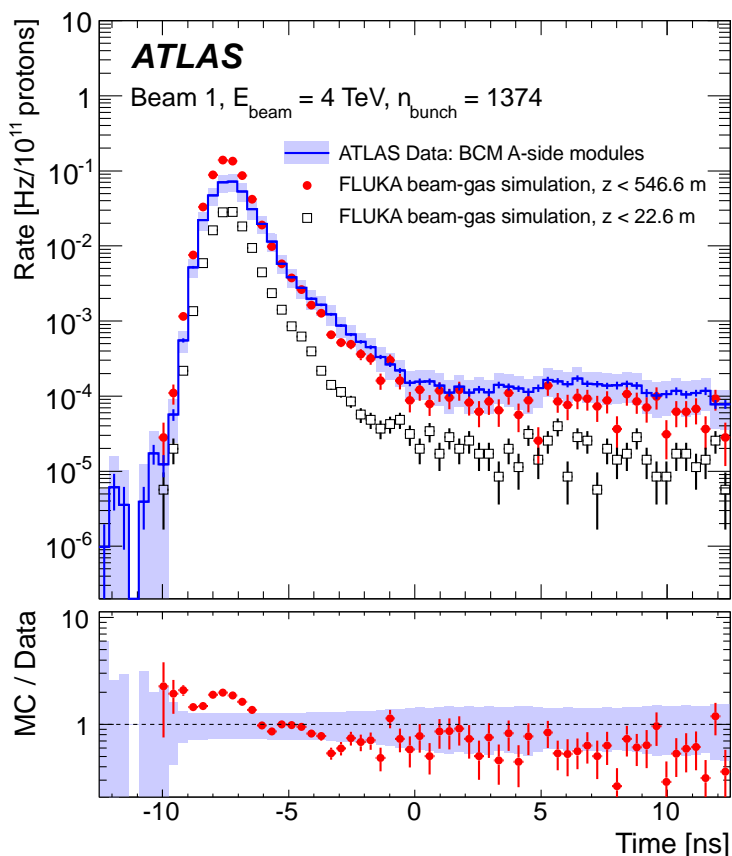
Figure 9. Comparison of the time distribution of BCM hits in ATLAS unpaired-bunch data (blue histogram) with FLUKA simulation (red circles). The bunch passes the IP at t = 0 \text{ ns} . The histograms show the early hits per upstream BCM module for events which have fired the BCM beam-background trigger in the beam-1 direction. The black open squares show the contribution from beam-gas events within the ATLAS experimental area z < 22.6 \text{ m} , while the red solid circles show the total, i.e. z < 546.6 \text{ m} . The errors shown on the simulation are statistical only. The blue band indicates the fill-to-fill and module-to-module variation of the data and the error bars show the uncertainty in the mean value. The lower panel shows the ratio of simulation to data, taken between the red circles and the blue histogram. Only data from the first ten minutes of ATLAS data-taking in each LHC fill are considered.
