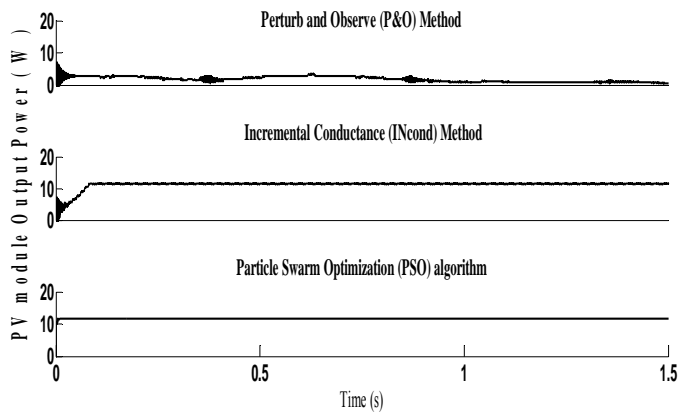
Fig. 12 The PV module output power (w) simulated with the MATLAB model at 200kw/m 2 , 25°C.
