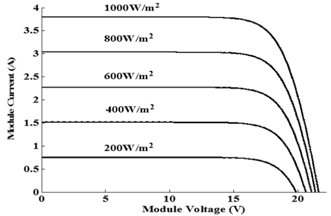
Fig. 3 I-V Characteristics with different irradiance values and a constant temperature ( 25^{\circ}\text{C} ).
